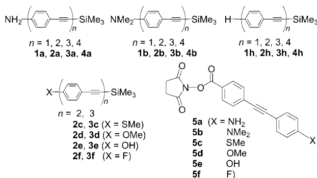
Figure 1. Structures of oligo(arylene-trimethylsilylethynylene)s and NHS-capped diphenylacetylenes.
