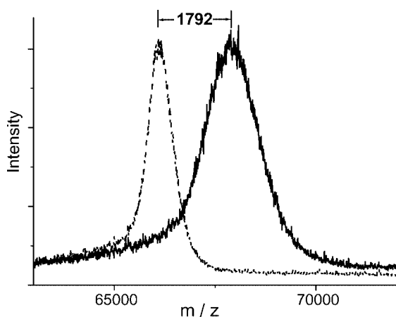
Figure 8. MALDI-TOF mass spectra of 5a -HSA conjugate (—) and HSA (----) ( \Delta m/z gives a labeling ratio of 7.6:1).
