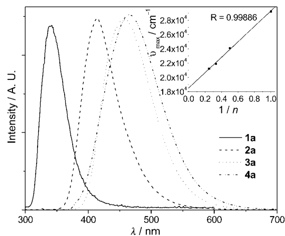
Figure 3. Emission spectra of 1a–4a in dichloromethane at 298 K (concentration = 2 \times 10^{-5} \text{ mol dm}^{-3} , \lambda_{\text{ex}} = 280–360 nm). Inset: plot of \tilde{\nu}_{\text{max}} [ \text{cm}^{-1} ] vs. 1/n .
