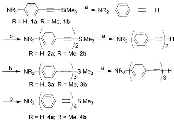
Scheme 1. Synthesis of 1a–4a and 1b–4b : a) 1.1 equiv. of KOH in MeOH/THF, 25 °C, 4 h; b) Pd(PPh_3)_2Cl_2 (2 mol-%), CuI (1 mol-%), 1-iodo-4-(trimethylsilylethynyl)benzene (0.91 equiv.), and NH_4Et in THF, 25 °C, 24 h.
