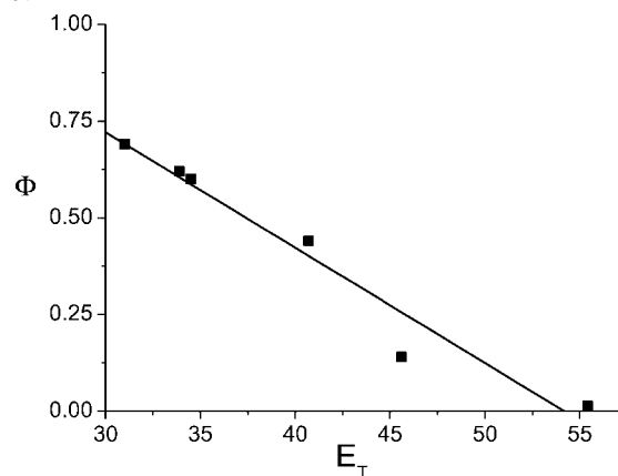
Figure 5. Plot of emission quantum yield for 2b in various solvents against the E_T value.
