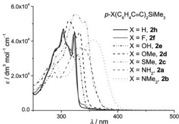
Figure 6. UV/Vis absorption spectra of 2a–2f and 2h in dichloromethane at 298 K.
