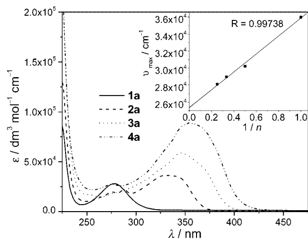
Figure 2. UV/Vis absorption spectra of 1a–4a in dichloromethane at 298 K. Inset: plot of \tilde{\nu}_{\text{max}} [ \text{cm}^{-1} ] vs. 1/n .
