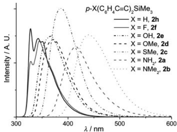
Figure 7. Emission spectra of 2a–2f and 2h in dichloromethane at 298 K (concentration = 2 \times 10^{-5} \text{ mol dm}^{-3} , \lambda_{\text{ex}} = 280\text{--}360 nm).
