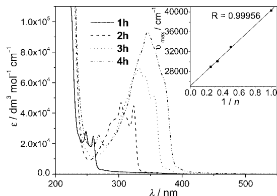
Figure 4. UV/Vis absorption spectra of 1h–4h in dichloromethane at 298 K. Inset: plot of absorption maximum in \tilde{\nu}_{\max} [ \text{cm}^{-1} ] vs. 1/n for \text{H}(\text{C}_6\text{H}_4\text{C}\equiv\text{C})_n\text{SiMe}_3 ( 1h–4h ).
